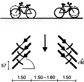
⑧ Staggered, herringbone formation
